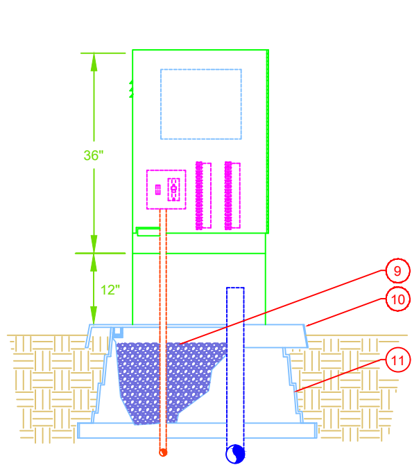
STRONGBOX FRONT ENTRY WITH STRONGBOX QUICKPAD.
