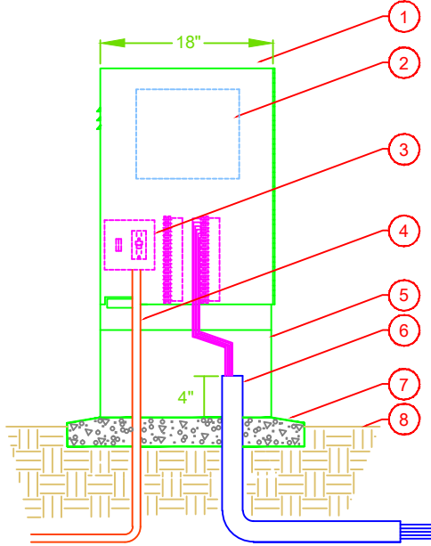
STRONGBOX FRONT ENTRY WITH CONCRETE PAD
