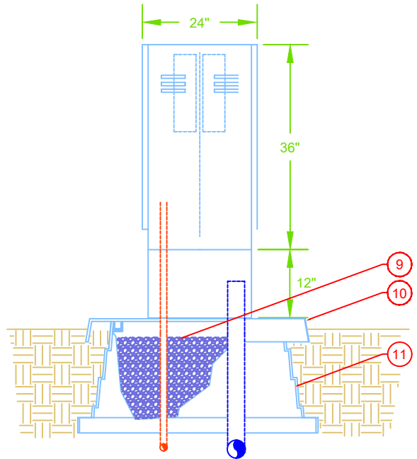
STRONGBOX DOUBLE DOOR ENCLOSURE (SIDE VIEW)
